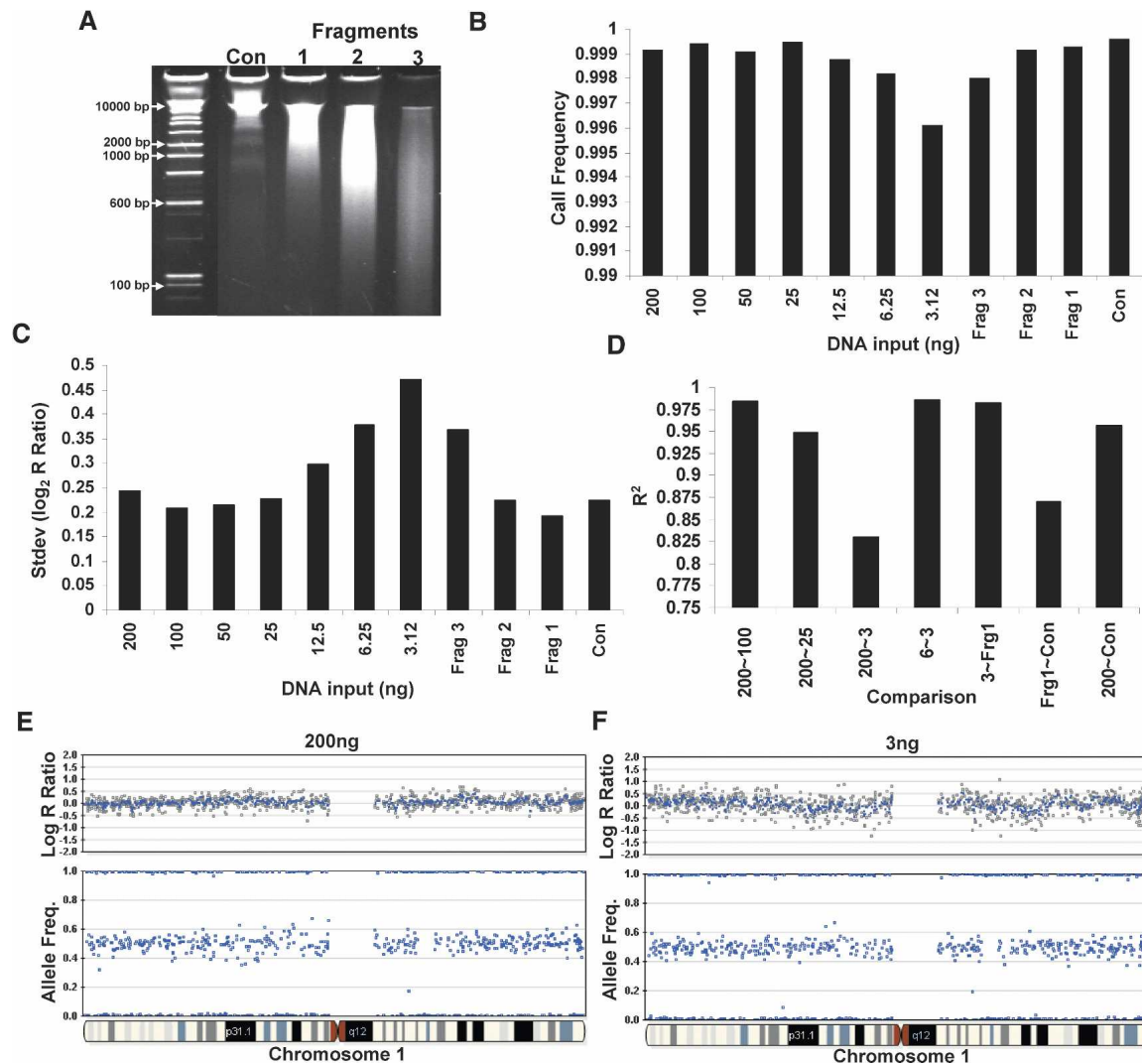
Figure 6. Effect of gDNA quantity and fragmentation length on SNP-CGH data. SNP-CGH data quality as a function of the quantity and fragmentation length of gDNA in the amplification reactions was tested using a multisample 10K BeadChip format. (A) Various lengths of fragmented DNA were used as starting input for the whole-genome amplification reaction (Fragments 1, 2, and 3). (B) The call rate is relatively insensitive to input amount across the entire range of 200 ng to 3 ng or fragment length. The call rates for input DNA ranging from 25 to 200 ng were all above 0.999, and the call rates for the 3–12.5 ng were all above 0.996. (C) Genomic DNA was titrated from the standard 1 \times input (200 ng in a one-quarter scale reaction) down to 1/64 th input (3 ng in a one-quarter scale reaction) as well as Fragments 1, 2, and 3. As the levels of input DNA decreased, the variability in the \log R ratio noticeably increased, whereas the allelic ratio was relatively insensitive to input amounts. (D) The R^2 correlation between samples remains high when similar amounts of gDNA are used for input regardless of whether it falls into either high or low levels; however, the R^2 decreases dramatically between inputs that differ substantially in amount. (E) An example genome profile from chromosome 1 showing both the \log R ratio and AF from the sample using 200 ng of input DNA. (F) The same plot as in E but with 3 ng of input DNA. Notice the slight increase in \log R ratio variability with the lower amount of DNA input.
