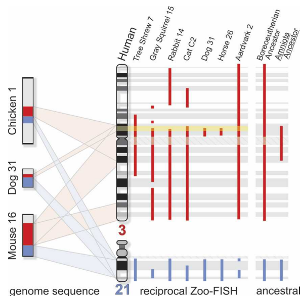
Figure 2. Comparisons of chicken, dog, and mouse genome sequence alignments to the human genome ( http://www.ensembl.org ) and Zoo-FISH data delineate an ancestral Amniota chromosome. Contiguous syntenic associations of human chromosome homologs 3 and 21 (top) are found in the genome sequence data indicated to the left of the human chromosome ideograms as well as in all of species analyzed by reciprocal Zoo-FISH. The vertical bars to the right of the G-banded human chromosome ideogram indicate the extent of the conserved segments displaying the syntenic associations in the selected species and chromosomes listed on top. Homologies to human chromosomes are identified by color: red (HSA3), blue (HSA21). Note that the intersection of homologous segments of human chromosome 3 in chicken, mouse, dog, and the horse (highlighted in yellow) indicate the ancestral fusion point of HSA3 to HSA21 in 3p12.3 (Froenicke 2005). Small genome alignment gaps inside conserved segments have been omitted for the sake of clarity. Similar agreements between chicken/human genome alignments and Zoo-FISH can be presented for the ancestral boreoeutherian associations HSA7/16, 14/15, and 16/19 (Supplemental Fig. 2). All three of these associations are missing in the bioinformatic model (Hillier et al. 2004; Bourque et al. 2005).
