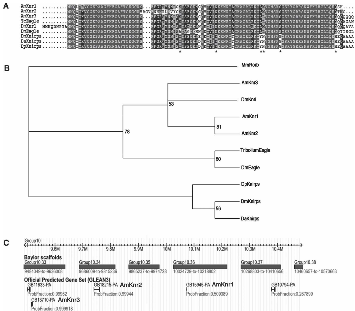
Figure 2. The honey bee genome contains three knirps -related genes. (A) Amino acids sequence comparison of the Zn finger domain from Knirps-related proteins including those predicted from the honey bee genome sequence. Asterisks indicate residues that are conserved in kni but not egon proteins; (Dp) Drosophila pseudoobscura . (B) Phylogenetic analysis of the Cys–Cys finger domains from Knirps-related proteins. kni from D. melanogaster forms a clade with kni proteins from other Drosophila species. (C) Genomic location of honey bee knirps -related genes. The three predicted knirps -related genes ( knr1 , knr2 , and knr3 ) are clustered on Baylor scaffold group 10.
