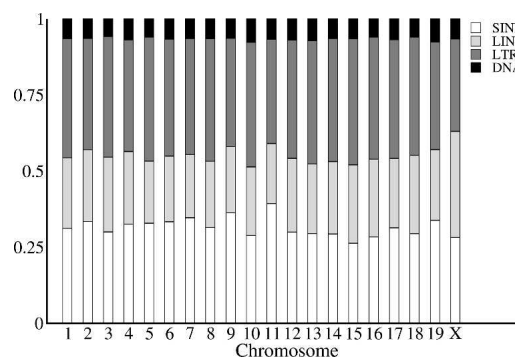
Figure 1. Proportion of total sequence per mouse chromosome contributed by each repeat class.
