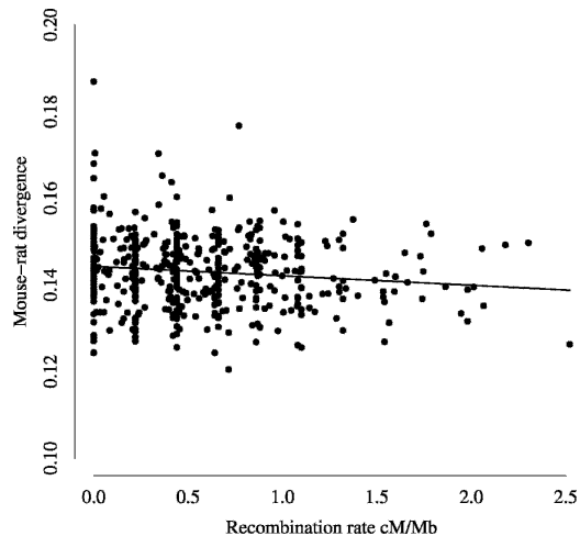
Figure 6. The relationship between mouse–rat divergence and the mouse recombination rate average across 5-Mb windows. The equation of the regression line shown was estimated as y = 0.144 - 0.002x .
