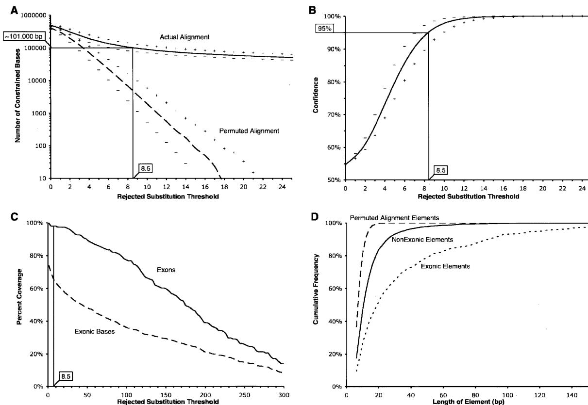
Figure 2. Confidence and sensitivity of GERP as a function of the rejected substitution threshold used to identify constrained elements. (A) Number of constrained element bases identified in the real alignment (solid line) and permuted alignments (dashed line). (B) Confidence is defined as the number of constrained element bases in the actual alignment divided by the sum of the constrained element bases in the actual and permuted alignments (see Methods). In A and B, the curves indicated with “+” and “-” characters result from analyses using a neutral rate estimate that is 10% greater or less, respectively, than the estimate of 3.85 neutral subs/site. A vertical black line marks the RS score threshold of 8.5 (corresponding to a confidence of ~95%). (C) The fraction of exons that overlap at least one constrained element (solid line), and the fraction of exonic bases within a constrained element (dashed line). (D) Cumulative frequencies of the sizes of constrained elements at an RS of 8.5 or greater, with permuted alignment elements (heavy dashed line), exclusively nonexonic constrained elements (solid line), and exonic elements (light dashed line).
