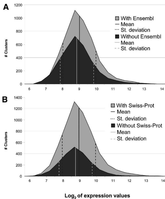
Figure 2. (A) Comparison of log 2 expression value distributions for T-clusters with and without overlaps with Ensembl gene predictions. The graph also depicts mean and standard deviation values for the corresponding distributions. (B) Comparison of log 2 expression value distributions for T-clusters with and without homology hits in the SWISS-PROT knowledgebase; mean and standard deviation values are also shown.
