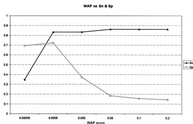
Figure 2. Performance of Footer in relation to the WAP threshold. This graph presents the sensitivity (black line) and specificity (gray line) over all promoter regions analyzed (see text). According to this graph, Footer performs best on a WAP threshold of 0.05%.
