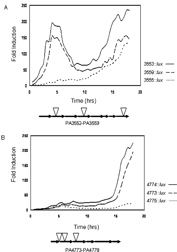
Figure 2. Induction of the PA3552–PA3559 and PA4773–PA4778 operons under Mg^{2+} limitation. The PA3552–PA3559 likely encodes an LPS modification operon that is strongly induced within hours of growth in Mg^{2+} -limiting medium. (A) Transcriptional luxCDABE fusions to PA3553, PA3555, and PA3559 are shown. The PA4773–PA4778 operon that encodes pmrAB is strongly induced in the late stages of growth in Mg^{2+} -limiting medium. (B) Transcriptional luxCDABE fusions to PA4773, PA4774, and PA4775 are shown. Luminescence (RLU) and OD_{620} were measured every 30 min throughout growth. All luminescence values were divided by the OD_{620} values to correct for growth and the ratio of normalized relative light units (RLU) in low to high Mg^{2+} conditions are plotted. All values shown are the mean of triplicate samples. Standard deviations were within 10% of the means.
