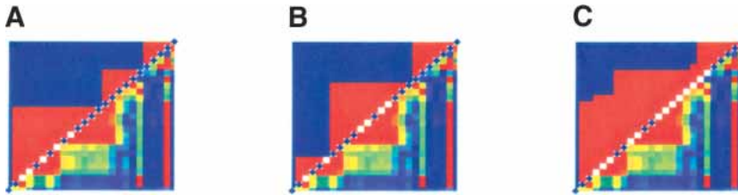
Figure 1 The three panels display a region of Chromosome 22. The lower triangle of each panel shows the LD between pairs of SNPs, where red denotes high LD and blue low LD. The upper triangles show the pairs of SNPs where one is used to predict the other. (A,B) The haplotype blocks as determined by two different runs of the block detection method of Gabriel et al. (2002). (C) The neighborhoods determined from taking the union of all possible Gabriel et al. blocks in the interval. The diamonds on the diagonal display the tagging SNPs selected for the three sets, using the algorithm of Zhang et al. (2003a) for the first two figures and the algorithm presented in this paper for the third figure.
