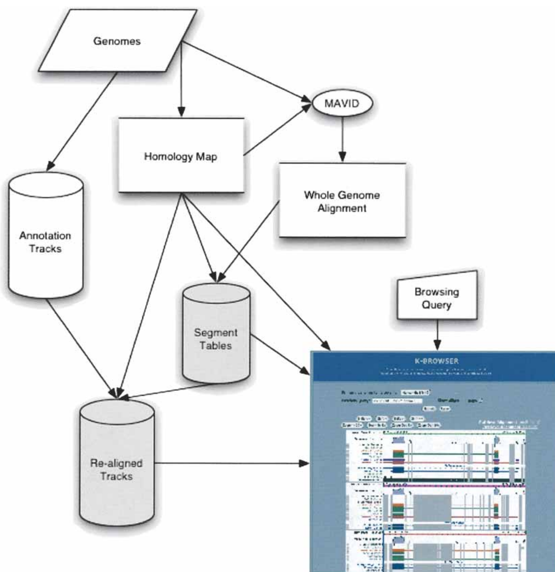
Figure 1 Schematic diagram of the K-BROWSER infrastructure. K-BROWSER builds two new databases (shaded) in addition to the standard annotation track database obtained from UCSC. These databases are based on a whole-genome alignment constructed using a homology map (in our case the blocks were aligned with the MAVID program). Using the segment tables and realigned tracks, a user query can be rapidly converted into a K-BROWSER figure.
