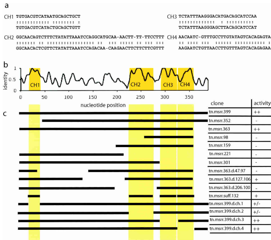
Figure 4. Deletion analysis of the minimally sufficient regulatory region. (a) The CHAOS algorithm returns four major regions of local conservation between C. savignyi and C. intestinalis . Note that this level of conservation stands out over neutrally evolving regions. (b) Plot of sequence identity between the C. savignyi and C. intestinalis TnI enhancer regions. The yellow shaded boxes represent the four CHAOS matches. (c) Horizontal lines denote sequence present in the constructs, activity is noted as in Figure 3. CHAOS matches CH1, CH2, and either of CH3/CH4 are necessary for expression of lacZ reporter in larval tail muscle. Concatenation of the four CHAOS matches is sufficient for weak lacZ expression.
