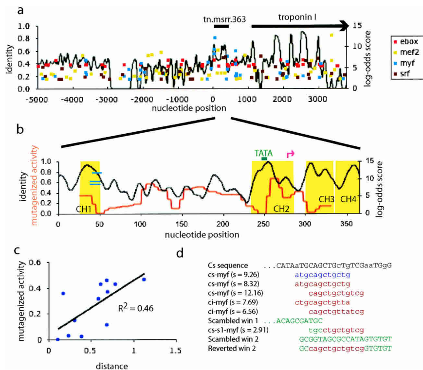
Figure 5. Conservation, predicted binding sites, and activity upon mutagenesis in the TnMSRR. (a) Plot of predicted binding sites for four common vertebrate muscle regulators for the TnI locus. The right y-axis shows the log-odds score of the site. The black line plots sequence identity (left y-axis) between C. savignyi and C. intestinalis . The location of the enhancer (tn.msrr.363) is shown. (b) Plot of conservation versus activity upon mutagenesis, with predicted binding sites. The left y-axis is sequence identity (black) and activity upon mutagenesis (red), and the right y-axis is the log-odds score of predicted sites. The black line plots sequence identity between the C. savignyi and C. intestinalis enhancers. The red line represents the activity (number of embryos staining/total embryos) of the lacZ reporter when a 20-bp window spanning that position is randomized. The yellow shading represents CHAOS hits, the green line is a conserved TATA-box, the pink arrow is the predicted transcription start site, and the blue lines are the three myf predictions. (c) Scatterplot of activity upon mutagenesis versus distance. The distance within each 20-mer is calculated by Kimura's two-parameter model. Mutagenized windows with activity >50% are not included, nor are poorly aligned sequences. (d) Predicted myf sites in C. savignyi and C. intestinalis , aligned with the two relevant scrambled windows. A predicted site remains in scrambled window 1, which retains activity, and no sites are predicted in scrambled window 2, which disrupts activity. Reverting one of the predicted sites back to wild type restores function (reverted window 2). Sequence of C. savignyi (Cs) is shown on top, with capital letters indicating identity with C. intestinalis . Blue sites are predicted on the forward strand, red sites on the reverse. All images and sequences are archived for retrieval at http://mendel.stanford.edu/supplementarydata/johnson .
