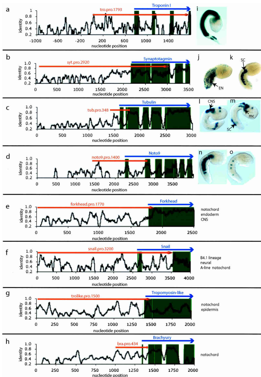
Figure 1. Five prime regions of eight Ciona loci. The black plots represent sequence identity between C. intestinalis and C. savignyi across each region. C. savignyi is the reference sequence for a–d, and C. intestinalis is the reference sequence for e–h. Green vertical bars correspond to annotated C. intestinalis exons. Blue arrows indicate direction of transcription of each gene. The red arrows indicate the native sequence present in the promoter fusion construct. Each promoter fusion construct contains significant regions of similarity between the two species. Expression patterns for C. savignyi constructs (i–o). Troponin I is strongly expressed in the tail muscle (i), Synaptotagmin is expressed in various neural lineages, including epidermal neurons (EN) (j) and spinal cord (SC) (k), \alpha -tubulin is expressed in various tissues, including central nervous system (CNS) (l) and spinal cord (SC) (m), and ectopic expression frequently occurs in the mesenchyme (MC) (m), Noto9 is expressed specifically in the notochord (n, o). All embryos were fixed at the mid-late tailbud stages. Electroporated embryos always exhibit mosaic staining patterns. A variety of typical images are archived at http://mendel.stanford.edu/supplementarydata/johnson .
