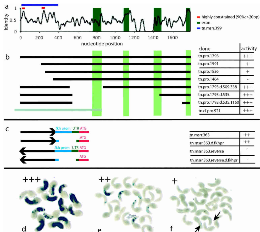
Figure 3. Activity of Troponin I-lacZ promoter constructs bearing various deletions, in context with sequence identity and exon structure of the locus. (a) Plot of sequence identity between C. savignyi and C. intestinalis in the promoter construct pro.1793 (cf. Fig. 1a). Green shading represents exons, the blue bar represents the MSRR, and the red bars indicate highly constrained regions (90% id; >20 bp). (b) Activity of deletion constructs, with tn.pro.1793; black lines denote sequence present in the constructs. The table lists activities of the constructs as explained below. Truncation of 329 bp from the 5'-end of the tn.pro.1793 construct completely eliminates expression in the tail muscle. Deletion of internal regions, including annotated exon 1, exons 1 and 2, and exons 1–3, has no effect. The gray line (tn.ci.pro.921) denotes the construct derived from C. intestinalis . (c) Activity of minimally sufficient regulatory region (MSRR) constructs. Fusion of the 5'-most 363 bp of tn.pro.1793 to a heterologous Forkhead basal promoter has strong activity. Deletion of the Forkhead basal promoter has no effect on lacZ expression. The reversed insert has no activity. (d–f) Relative activities of constructs. We classify constructs as (d) +++, representing 50%–100% animals staining, with many of the animals staining strongly in a majority of the tail muscle cells; (e) ++, representing 25%–50% of the animals staining in the tail muscle, and the minority of these staining a majority of the tail muscle cells; and (f) +, with <25% of the animals staining, and none of the animals staining the majority of the tail muscle cells; “–” indicates a construct that never showed staining. Constructs that were mostly “–” but stained weakly on a single occasion are denoted +/-.
