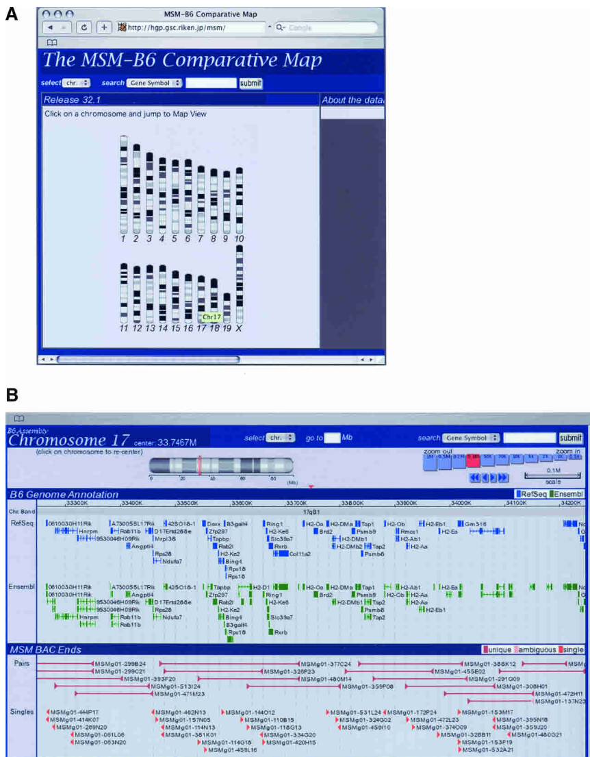
Figure 2. BAC contigs retrieved by the web-based clone screening system. By clicking a genomic region of interest on the chromosome map in the top menu, BAC contigs covering the corresponding genomic region can be viewed (A). The red triangles represent the 'unique paired-end' BAC clones; the pink triangles represent 'ambiguous' BESs. Locations of 'one-ended' BAC clones are shown by the orange triangles (B). Clone MSMg01-114N13 is an example of such 'one-ended' clones; its size is ~150 kb long, extending toward the centromere, and the clone was found to contain the Rps28 , Angptl4 , Rab11b , and 9530046H09Rik genes.
