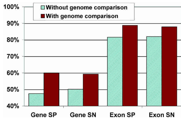
Figure 2. Accuracy of the gene prediction set generated without genome comparison and the final prediction set, which was generated using comparison to the Serotype A genome. The smoothed empirical intron length model was used in generating both sets.
