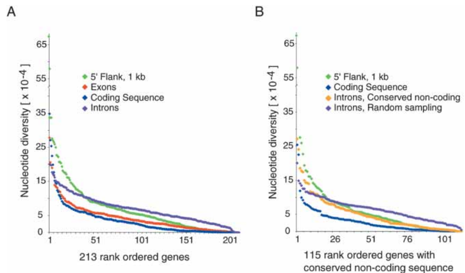
Figure 1 Rank order of nucleotide diversity ( \pi ) in conserved noncoding, exon, intron, CDS, and 5' flanking regions of the EGP genes. (A) Values are calculated for all 213 EGP genes for regions containing 1 kb 5' of the transcription initiation site (green, 174 kb), exons (red, 483 kb), coding sequence (blue, 312 kb), and introns (purple, 3.26 Mb). (B) \pi values are calculated for 115 EGP genes that had significant amounts of intronic conserved noncoding sequence (as described in Methods) for regions containing 1 kb 5' of the transcription initiation site (green, 91 kb), coding sequence (blue, 189 kb) and intronic conserved noncoding (orange, 170 kb), and randomly sampled intron (purple, 2.39 Mb). All categories were sorted independently before plotting. The randomly sampled intron category corresponds to the mean \pi value per gene obtained by 10,000 independent samplings of the same size range as the intronic conserved noncoding region for that gene. The average SEM for this sampling was 9.3E-06 with a minimum and maximum SEM of 3.12E-07 and 3.07E-05 , respectively.
