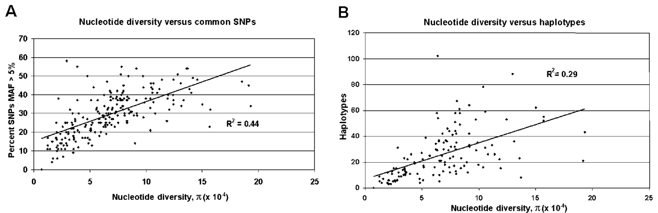
Figure 4 The relationship between nucleotide diversity and the number of common SNPs (A) or the number of inferred haplotypes (B) for 213 environmental response genes.
