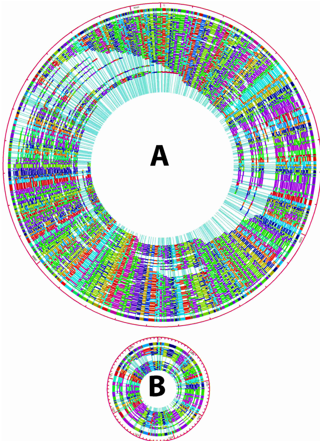
Figure 1 Whole-genome Eco RI optical map contigs of chromosome I and II of R. sphaeroides 2.4.1. (A) Chromosome I circular map contig. The outermost multicolored ring shows the consensus map calculated by Gentig. The consensus map was built from the shown underlying maps, obtained from individual DNA molecules, and represented here as multicolored arcs. Congruent restriction fragments, shown in the consensus map are denoted by common color; the color coding scheme is random to enhance contrast. Missing cuts are displayed as fragments that span across one or more cut sites in the consensus map. (B) Chromosome II circular map contig; display scheme is the same as (A).
