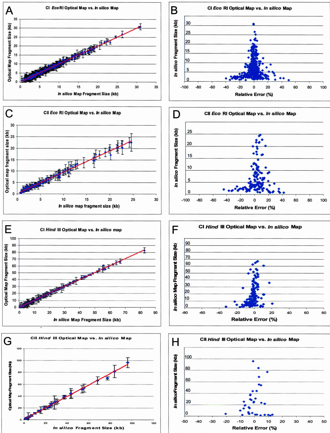
Figure 2 Comparisons of the HindIII and EcoRI optical maps of R. sphaeroides chromosome I (CI) and chromosome II (CII) to sequence data. (A) (CI EcoRI ), (C) (CII EcoRI ), (E) (CI HindIII ) and (G) (CII HindIII ) are the plots of optical map fragment sizes versus the in silico map fragment sizes from finished sequence. The error bars represent the standard deviation of optical map fragment size on the means. (B) (CI EcoRI ), (D) (CII EcoRI ), (F) (CI HindIII ), and (H) (CII HindIII ) show plots of the absolute error of optical fragment size versus sequence.
