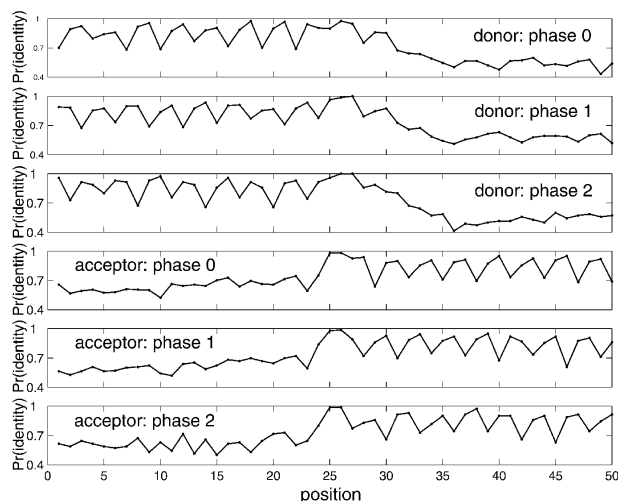
Figure 7 Conservative patterns at the splice sites of introns in different phases. The \text{Pr}(\text{identity}) on y-axis stands for probability of identity at each position on the alignment. Positions 26 and 27 in the donor site correspond to GT, the terminal residues of the intron at the 5' splice site, and positions 25 and 26 in the acceptor site correspond to AG, the terminal residues of the intron at the 3' splice site. It can be seen that exonic regions not only are more conserved than intronic regions, but also display phase-dependent conservative patterns, which agree well with the preferred substitution in the third codon positions in the coding regions.
