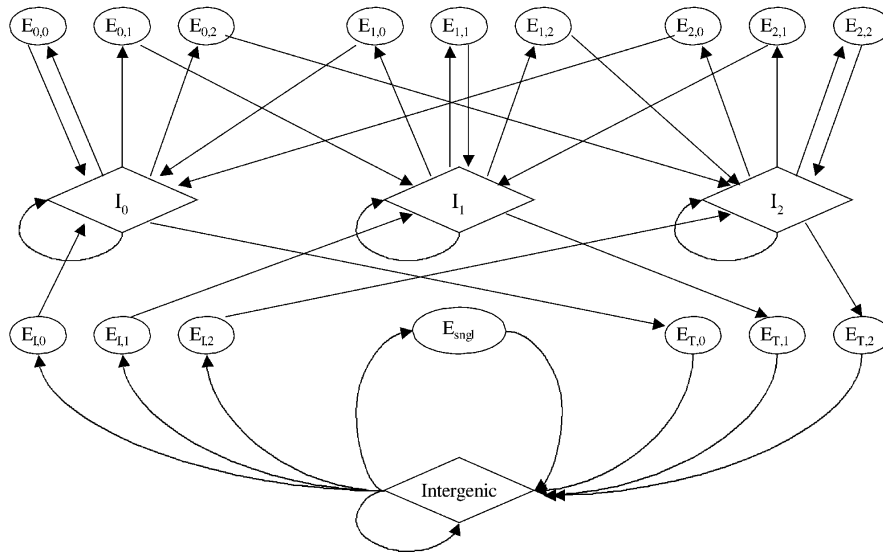
Figure 3 Generalized Hidden Markov Model of genomic sequence structure. Each oval or diamond represents a unit in the genomic sequence as follows: intergenic; E_{i,k} , k = 0, 1, 2 , three states for initial exons; E_{T,k} , k = 0, 1, 2 , three states for terminal exons; E_{sngl} , single exon genes; E_{i,l} , l = 0, 1, 2 , k = 0, 1, 2 , internal exons at reading frames l ; I_l , l = 0, 1, 2 , introns at reading frames l . Splice signals (donor and acceptor) and translational initiation and termination signals are subcomponents of exons and are not shown in the model. Promoters, 5' and 3' UTRs, poly(A) signals, and the complementary strand are not modeled. The length distribution of each coding state is modeled explicitly.
