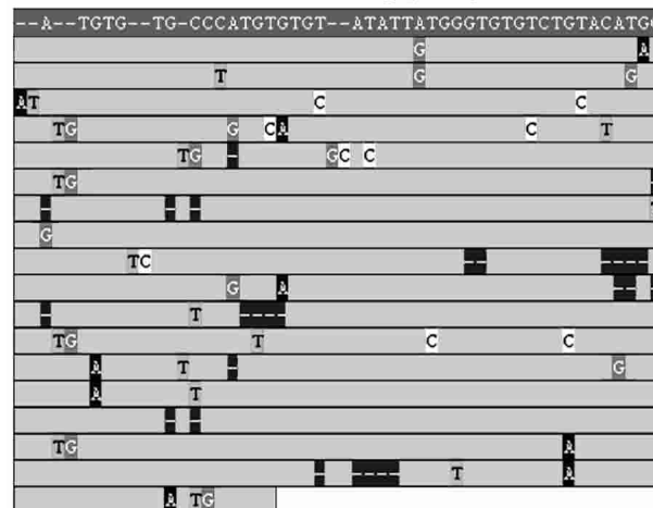
Figure 1 Multiple alignments of tandem repeats CEB252 and CEB233. In each alignment, the upper darker line is a consensus pattern for the basic unit, shown for reference, and the lighter lines are the individual copies, ordered from top to bottom as they occur in the repeat. Only differences with the consensus are shown. Heterozygosity for CEB252 is 0.6. Note several redundant patterns of mutation resulting in a high HistoryR score. Heterozygosity for CEB233 is zero. No clear organization of mutations resulting in a low HistoryR score.
