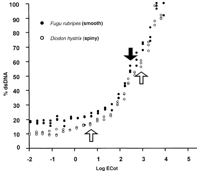
Figure 1 Cot curves for a tetraodontid (smooth) puffer, Fugu rubripes , and a diodontid (spiny) puffer, Diodon hystrix . Filled circles indicate F. rubripes data points, and open circles represent D. hystrix data points. Open arrows mark the Cot_{1/2} values of the D. hystrix repetitive (left) and single-copy (right) classes, at which half of those components are estimated to have renatured. The filled arrow indicates the Cot_{1/2} value of the single-copy component of the F. rubripes genome. The Cot_{1/2} value of the F. rubripes repetitive component is estimated to be -3.3 , and does not appear on this graph.
