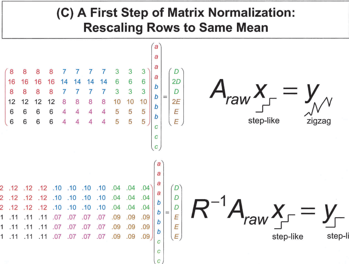
Figure 1 Overview of important parts of the biclustering process. (A) shows the problem: shuffling a gene expression matrix to reveal a checkerboard pattern associating genes with conditions. (B) shows how this problem can be approached through solving an “eigenproblem.” If a gene expression matrix A has a checkerboard structure, applying it to a step-like condition classification vector x will result in a step-like gene classification vector y . Moreover, if one then applies A^T to y , one will regenerate a step-like condition classification vector with the same partitioning structure as x . This suggests one can determine whether A has a checkerboard structure through solving an eigenvalue problem. In other words, if A has a (hidden) checkerboard structure, there exist some piecewise constant partition vectors x = v , and y = u , such that A^T A v = \lambda^2 v , and A A^T u = \lambda^2 u . (bottom quadrant of part B). Note that most eigenvectors v of the eigenvalue problem A^T A v = \lambda^2 v (symbolized by a zigzag structure) are not embedded in the subspace of classification (step-like) vectors x possessing the same partitioning structure, as indicated by a gray arrow protruding from this subspace (parallelogram). On the other hand, piecewise constant (step-like) partition eigenvectors v , are embedded in this subspace and are indicated by a green arrow. To reveal whether the data have a checkerboard structure, one can inspect whether some of the pairs of monotonically sorted gene and tumor eigenvectors v_i and u_i have an approximate stepwise (piecewise) constant structure. The outer product u_i v_i^T of the sorted partitioning eigenvectors gives a checkerboard structure. (C) shows how rescaling of matrix A can lead to improved copartitioning of genes and conditions.
