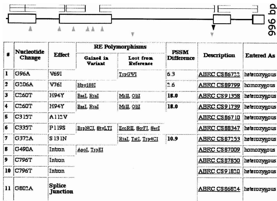
Figure 3 PARSESNP output for a typical ATP order. Users are provided a link to PARSESNP, which automatically analyzes mutations discovered. The graphical and tabular output from PARSESNP is shown. Near the top is a graphical view of the gene model; (boxes) exons, (lines) introns. Above the gene model is a Blocks protein conservation model. Below the gene model, triangles represent the location and type of induced change. These data are also summarized in tabular form below and on the nucleic acid sequence itself (data not shown). The effect of each nucleotide change is listed in the table. Missense changes are provided with a PSSM difference score by PARSESNP, in which mutations predicted to be damaging to the protein have positive scores, based on a scoring matrix generated from the protein conservation model (see http://www.proweb.org/glossary.html for a description of scoring missense changes). The restriction sites either gained or lost because of the induced polymorphism are listed. These sites serve as a tool for downstream genotyping applications.
