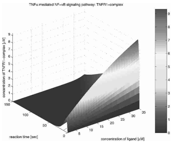
Figure 15 TNFR1 complex.
