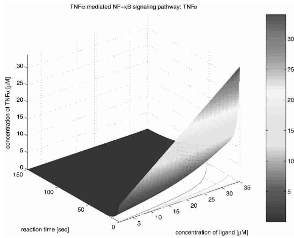
Figure 13 TNF \alpha .
