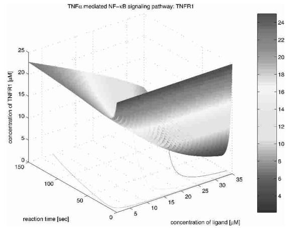
Figure 14 TNFR1.
