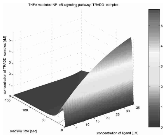
Figure 17 TRADD complex.
