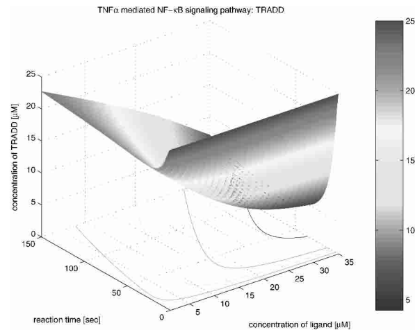
Figure 16 TRADD.
