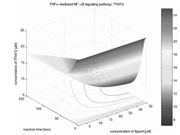
Figure 20 TRAF2.
