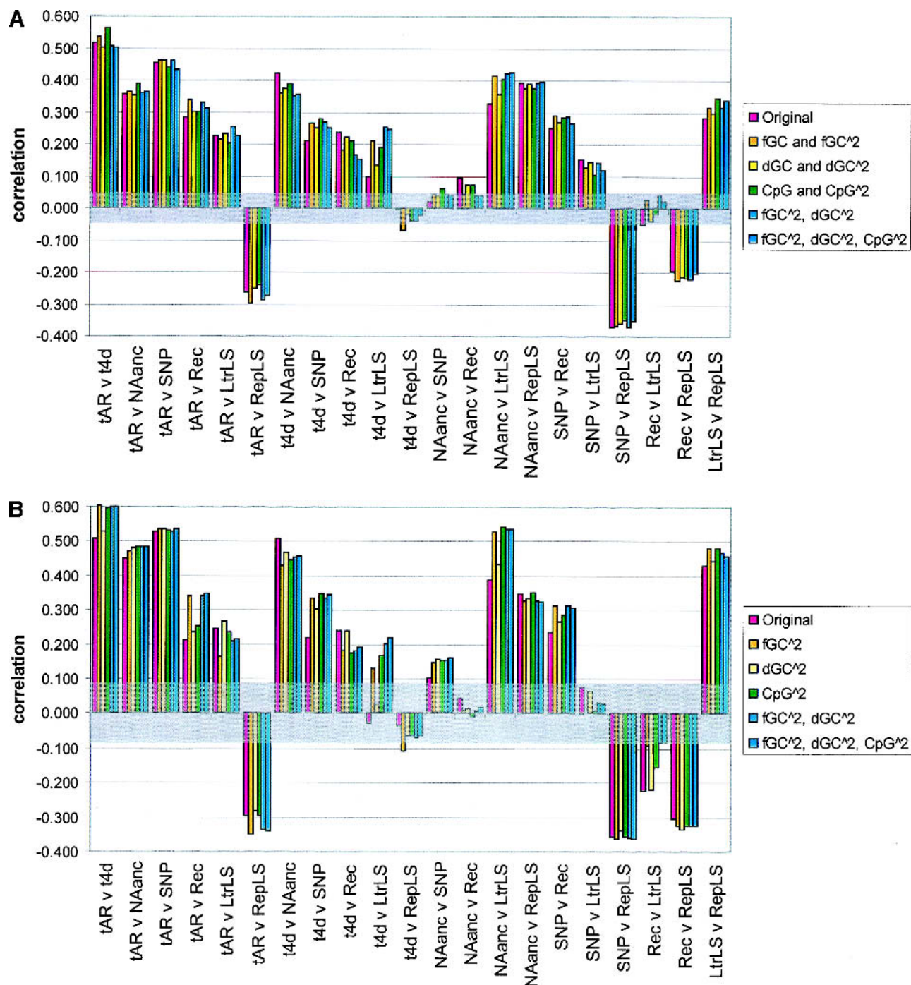
Figure 4 Pairwise correlations for various divergence measures, before and after correcting for the effect of GC content, difference in GC content between human and mouse, and CpG density in human. The seven divergence measures are neutral substitution rates in ancestral repeats ( t_{AR} , noted as tAR in the graph) and 4D sites ( t_{4D} , noted as t4d in the graph), deletion proxied by NA_{anc} , SNP density, recombination rate ( Rec ), and insertion proxied by density of lineage specific LTR repeats ( LtrLS ) and density of lineage-specific repeats in general ( Repls ). Correlations are plotted as bars for (1) original divergence measures (in red); (2) residuals from quadratic regressions on GC content (the regression terms are a constant intercept, fGC and fGC squared) (in gold, noted in the key as fGC^2 ); (3) residuals from quadratic regressions on change in GC content between human and mouse (the regression terms are a constant intercept, dGC and dGC squared) (in yellow, noted in the key as dGC^2 ); (4) residuals from quadratic regressions on CpG density (the regression terms are a constant intercept, CpG density and CpG density squared) (in green, noted in the key as CpG^2 ); (5) residuals from quadratic regressions on GC content and difference in GC content between human and mouse (the regression terms are a constant intercept, fGC , fGC squared, dGC , and dGC squared) (in lighter blue, noted in the key as fGC^2 , dGC^2 ); and (6) residuals from quadratic regressions on GC content, difference in GC content between human and mouse, and CpG density in humans (in darker blue, noted in the key as fGC^2 , dGC^2 , CpG^2 ) (A) The results for 1-Mb nonoverlapping windows; (B) the results for 5-Mb nonoverlapping windows. A transparent gray rectangle encompasses correlations for which the p -values fall above 0.050 (i.e., a correlation that is not significant at the 5% Type-I error level).
