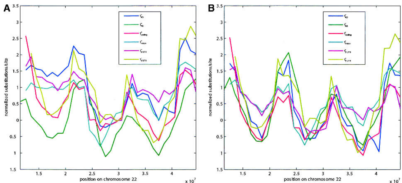
Figure 2 Variation in t_{4D} , t_{AR} , t_{intron} , t_{coding} , t_{3'UTR} , and t_{5'UTR} along human Chromosome 22 (A) and residuals of t_{4D} , t_{AR} , t_{intron} , t_{coding} , t_{3'UTR} , and t_{5'UTR} after quadratic regressions on human CG content along human Chromosome 22 (B). All values were calculated from 5-Mb overlapping by 4-Mb windows of the human–mouse alignment and were normalized using the genome-wide mean and standard deviation (denoted by superscript + in A and * in B). The normalization was done to ensure that all values have the same dynamic range.
