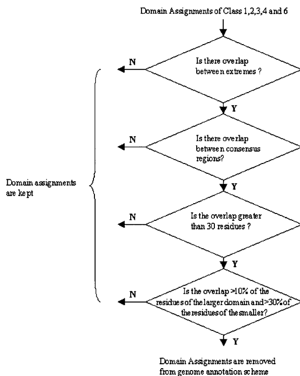
Figure 10 The Clean Assign Module's decision flowchart for deciding on acceptable overlaps between consensus regions with differing homologous superfamily assignments. The CATH domain assignments from domains in CATH classes 1, 2, 3, 4, and 6 (see Table 1) are analyzed by the decision tree.
