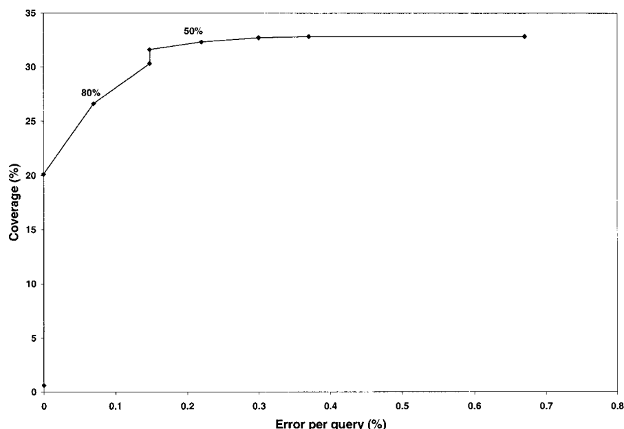
Figure 5 Error per query (%) by Coverage (%) obtained for one-to-one relationships. The coverage is measured using the CATH-35 sequences. This graph shows the percent coverage of true positives divided by the total number of possible assignments against the numbers of errors per query. These values are plotted for the differing percentages of the query domain (Q) in the alignment.
