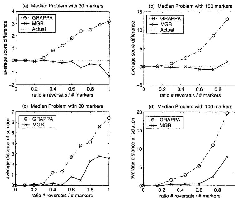
Figure 2. Comparison of MGR-MEDIAN and GRAPPA (three genomes equidistant from the ancestor). The genomes G_1, G_2, G_3 are obtained by k reversals each from the ancestral identity permutation 1\ 2\ \dots\ n ( n = 30 and n = 100 ). The simulations were repeated 10 times for every ratio \# \text{reversals} / \# \text{markers} = 3k/n . (a) and (b) show the average difference between the number of reversals on the tree recovered by the algorithm and the number of reversals on the actual tree (equal to 3k ). (c) and (d) show the average reversal distance between the solution recovered and the actual ancestor.
