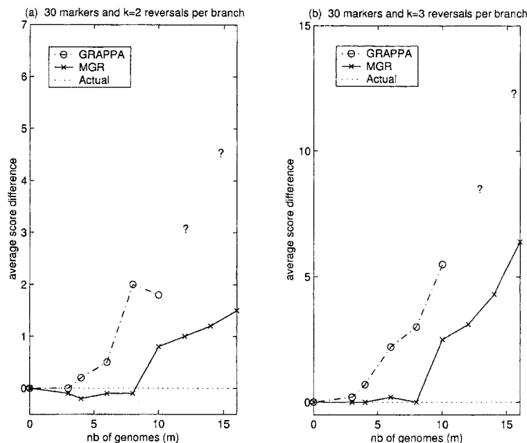
Figure 5. Comparison of MGR and GRAPPA ( m genomes each with 30 markers). The genomes G_1, G_2, \dots, G_m correspond to a subset of leaves from a complete unrooted binary tree on which we have performed k reversals on each branch. The simulations were repeated 10 times for every m . (a) and (b) show the average difference between the number of reversals on the tree recovered by the algorithm and the number of reversals on the actual tree when k = 2 and k = 3 , respectively.
