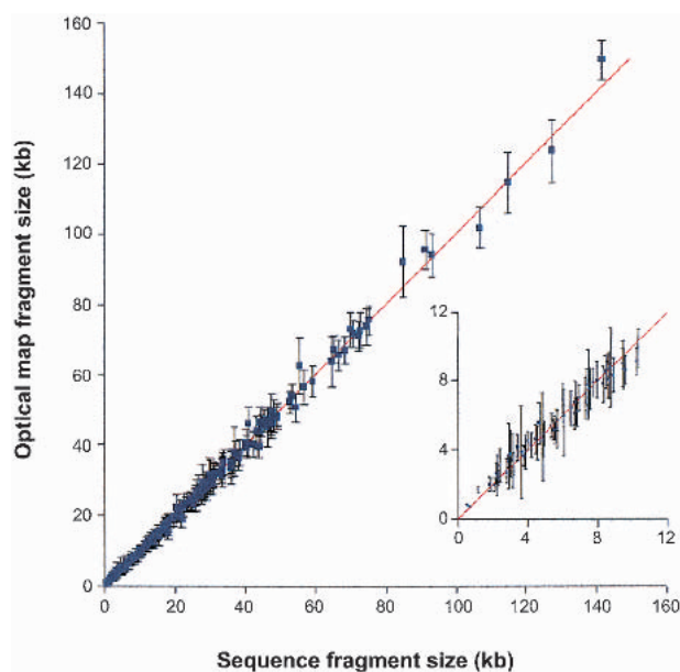
Figure 3 XhoI restriction endonuclease fragment sizing results for E. coli O157:H7 plotted against sequence data. The diagonal line is for reference. The error bars represent the standard deviation of the fragment sizes. (Inset) Fragment sizes <10 kb.
