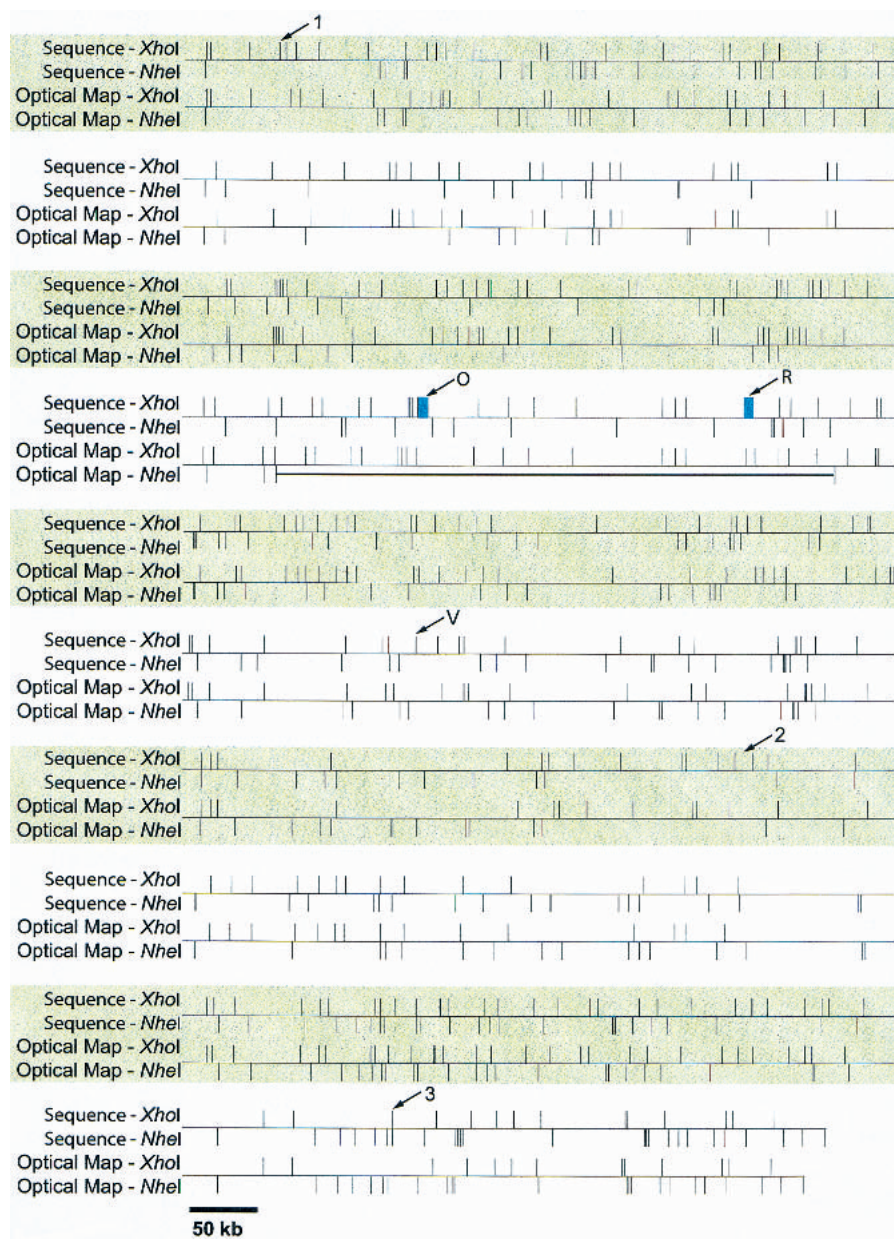
Figure 4 Alignment of map and sequence data. The use of sequence information to link single-enzyme optical maps. The composite optical map was generated by normalizing the single-enzyme maps to be the same size. The resulting multienzyme map was aligned with the map predicted from sequence. The thick black horizontal line denotes a missing region in the NheI optical map. The arrows show discrepancies between sequence and the optical maps. These discrepancies correspond to those in Figure 2b. The blue rectangles denote gaps in the sequence data compared to the XhoI optical map.
