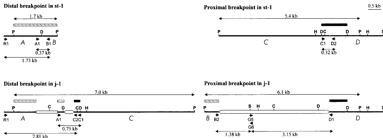
Figure 1 Physical map of the distal and proximal 2j breakpoint regions in the st-1 and j-1 lines. Thick lines represent the single-copy A , B , C , and D sequences. TE insertions are represented as empty boxes. Hatched and black rectangles correspond, respectively, to the AB and CD probes used for the Southern hybridization analysis. Small arrows represent primers used in the PCR amplification. Some of the restriction sites found in this region are shown: C , Clal ; D , Dral ; H , HindIII ; P , PstI ; S , SalI .
