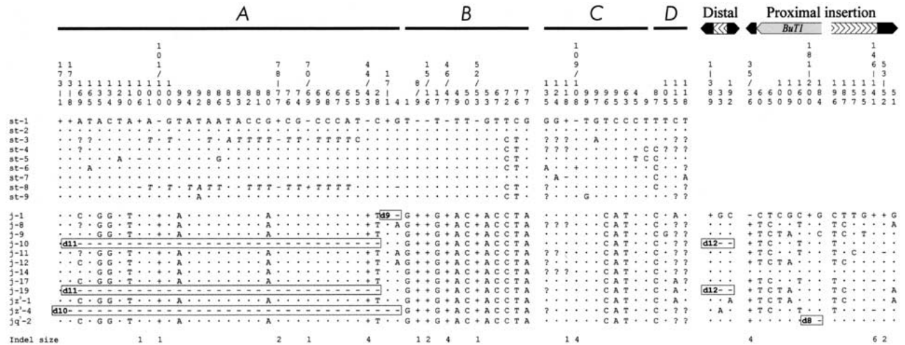
Figure 3 Nucleotide polymorphism at the breakpoint regions of inversion 2j . Nucleotide position is represented above the sequences. The breakpoints are taken as start point of A , B , C , D , distal breakpoint insertion, and proximal breakpoint insertion sequences. Nucleotides identical to the first sequence are indicated by a dot and missing data by a question mark. Deletions and insertions are indicated by minus and plus signs, respectively, and their size in base pairs is shown below. Gross deletions affecting the sequenced regions are named as in Fig. 2 and are included in rectangles. TE insertions and target site duplications are not shown. In 2st lines there is a 18-bp stretch between A and B sequences resembling Galileo footprints (Cáceres et al. 1999) that is not represented here either. Positions A65 to A101 in st-3 and st-8 accumulate multiple nucleotide changes with regard to the other lines and are shown in italics.
