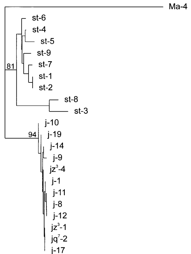
Figure 4 Neighbor-joining phylogenetic tree of the breakpoint sequences of inversion 2j based on the A , B , C , and D sequence data for the nine 2st and 12 2j Drosophila buzzatii lines. The Ma-4 Drosophila martensis line was used as outgroup. Bootstrap values in percentage out of 500 replicates are indicated for the main nodes.
