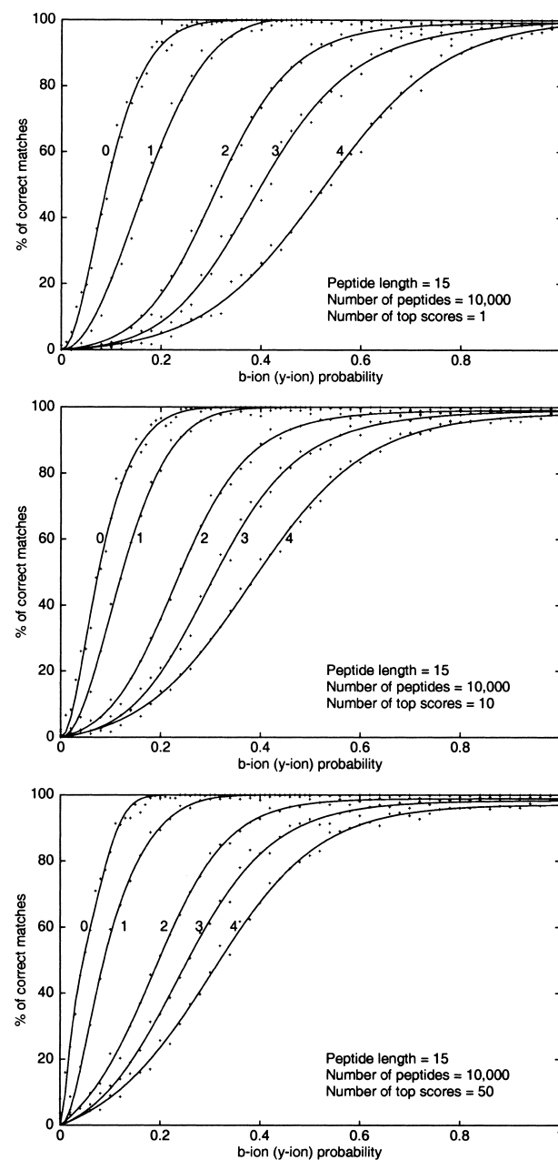
Figure 6 Database search success rate of spectral alignment approach for the simulated spectra. A match is successful if one of indicated top-scored spectra matches a correct peptide. The number next to a curve is the number of mutated amino acids k .
