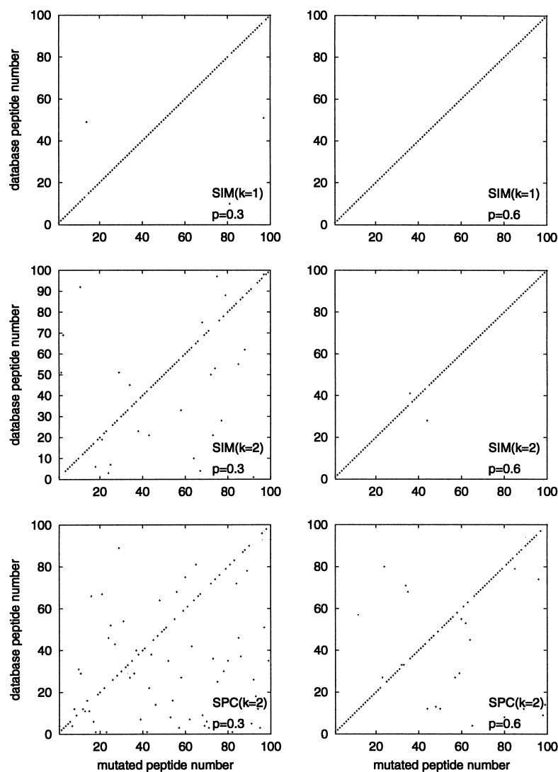
Figure 4 The matching spectra of mutated peptides with peptides in a small database (100 peptides) at different values of spectral quality p and number of mutations k . The first two pair of plots describe matching with SIM_1 and SIM_2 similarity scores for k=1 and k=2 mutations. The third pair of plots describes matching with the Shared Peaks Count (SPC). Crosses represent best matches, dots represent second-best matches. A cross at position (i, i) on the main diagonal represents the correct matching of spectra i and peptide i .
