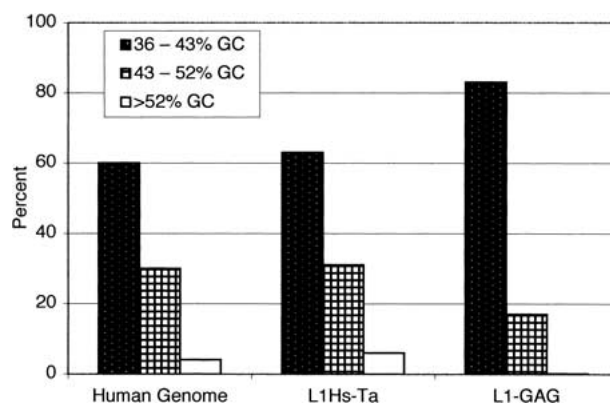
Figure 5 Distribution of L1 insertions in genomic DNA of different GC content. The GC content of the 3' flanks of L1 insertions was calculated starting 150 bp after the poly(A) addition signal. Each insertion was assigned to bins of either 36%–43% GC (stippled), 43%–52% GC (checkered), or >52% GC (open box).
