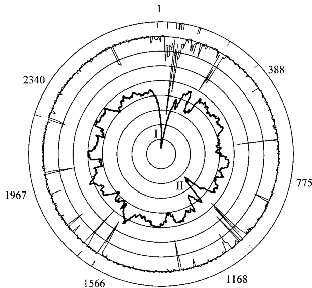
Figure 6 Circular representation of the Halobacterium NRC-1 chromosome showing the GC composition of ORFs, \chi -squared analysis, and location of IS elements. The outer scale refers to ORF identification numbers. Bars associated with the outmost circle denote the position of the chromosomal IS elements. \chi -squared analysis is plotted as a thin black line, and average GC content of ORF is the innermost plot in darker black, each against their relative position on the circular map. The Roman numerals I and II inside the plot indicate relatively AT-rich islands.
