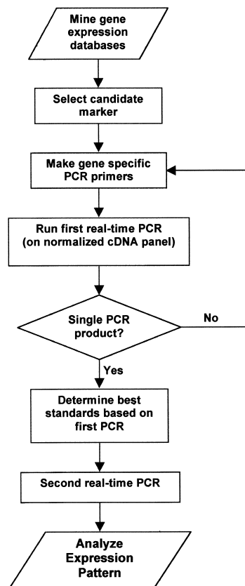
Figure 1 Process for finding candidate tumor markers, using fluorescent-PCR expression comparison (F-PEC). Genes overexpressed in tumors are mined from gene-expression databases. A normalized cDNA panel is used to rapidly compare expression levels in malignant and normal tissues. The process requires an initial PCR to determine the specificity of the primers, the product melting temperature, and the expression range of the tested samples. The highest-expressing sample from the first PCR is serially diluted to create a standard curve for a second PCR, yielding information on the relative expression over several orders of magnitude.
