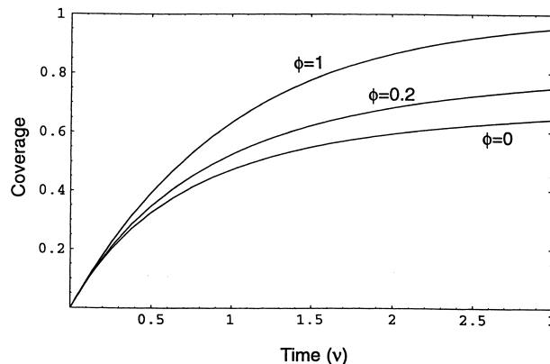
Figure 3 Coverage versus time. Coverage is asymptotic to the jamming limit, which varies with the allowed overlap \phi .
