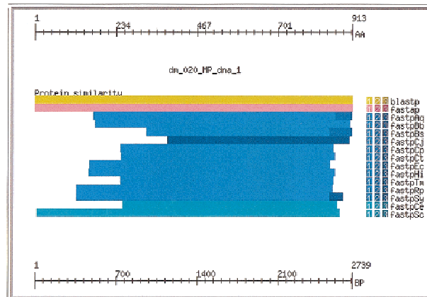
Figure 6 Evidence summary for DNA mismatch repair protein showing matches in 11 bacterial genomes (blue) and 2 eukaryotic genomes (cyan).
