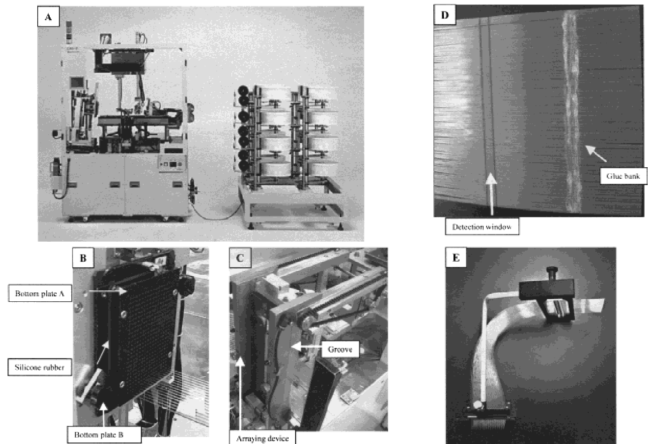
Figure 7 Photographs of the RISA capillary array assembler (CAS). (A) The RISA capillary array assembler. (B) Sixteen capillaries penetrating the silicone plate. (C) The arraying device. (D) Capillary sheet. (E) The 384-capillary cassette.
