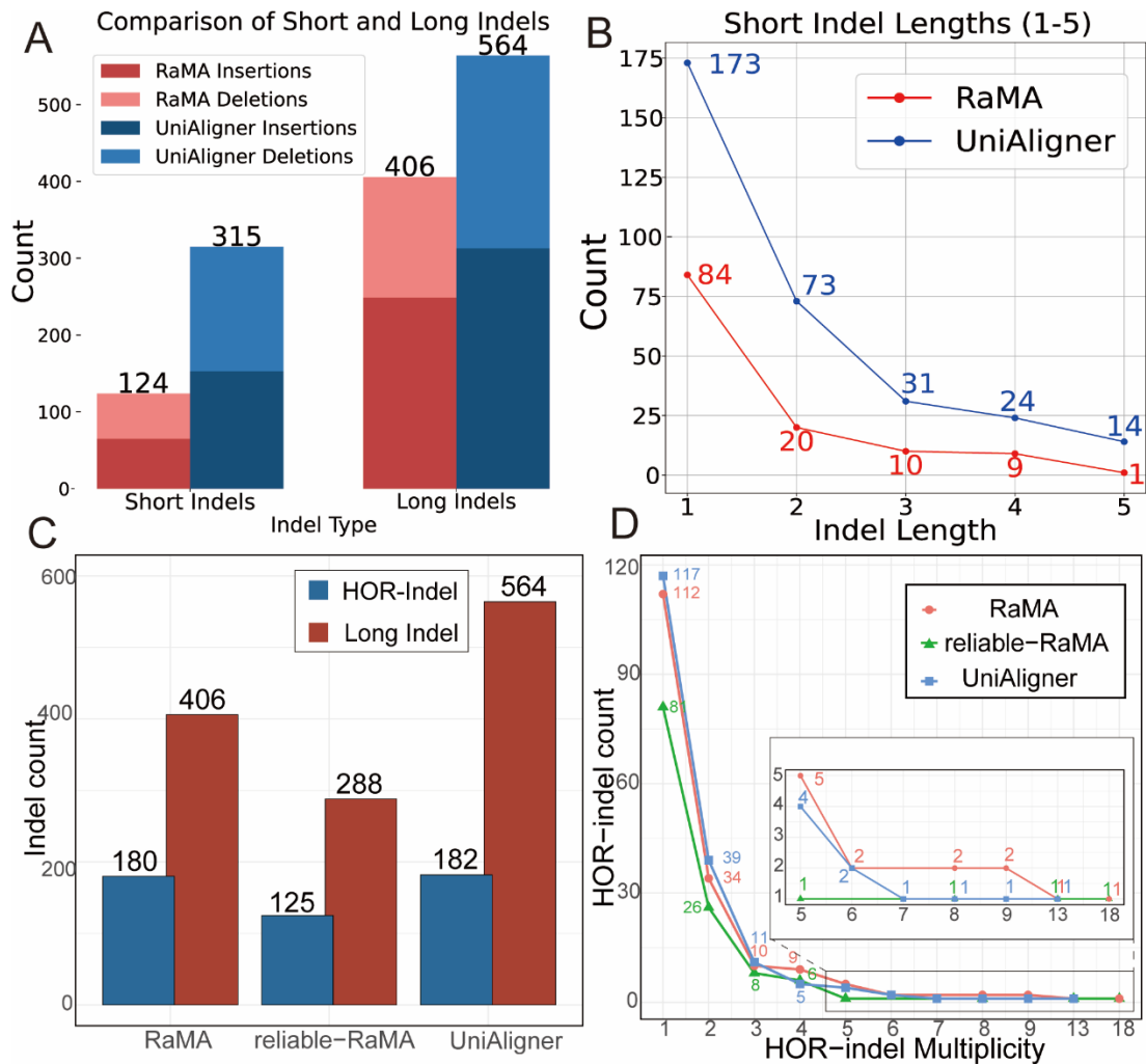
Fig 3 Figures A-D show the statistical results of centromere alignment on the X Chromosome for CHM13 and CHM1: (A) Comparison of the number of short and long indels, as well as insertions and deletions, in the alignment results of the two methods. (B) Comparison of the distribution of short indels ( \leq 5 bp) by length in the alignment results of the two methods. (C) Comparison of the number of long indels and HOR-indels in RaMA alignment results, reliable regions of RaMA based on the rare match and the UniAligner alignment results. (D) Distribution of the multiplicity of HOR indels in RaMA alignment results, reliable regions of RaMA based on the rare match and the UniAligner alignment results.
