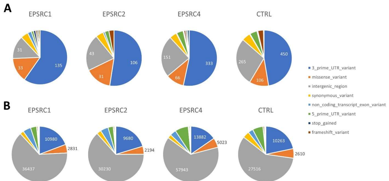
9 Figure 7: Breakdown of variant annotations for (a) scu-variants and (b) rare positive variants
