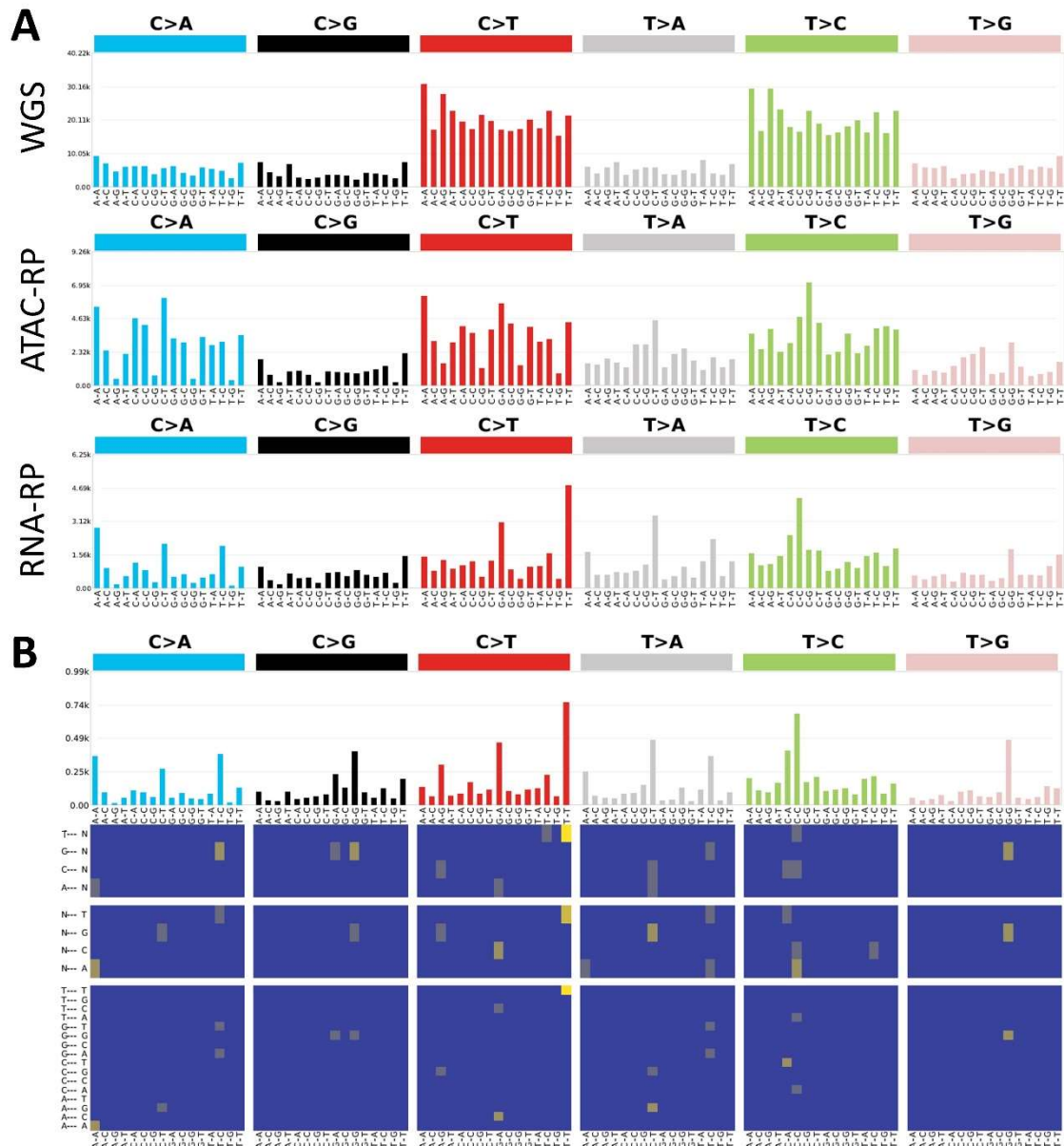
Figure 5: SBS 96 trinucleotide mutation breakdown for (a) common ground-truth, scATAC-RP, and scRNA-RP variants as seen in EPSRC1 which is representative of the group trend, and (b) the SBS1536 breakdown of scRNA-RP variants in exonic regions only, demonstrating that the signature is maintained in exonic regions and is characterized by repeat-extensions of all base patterns. Images were generated using the SigProfiler suite.
