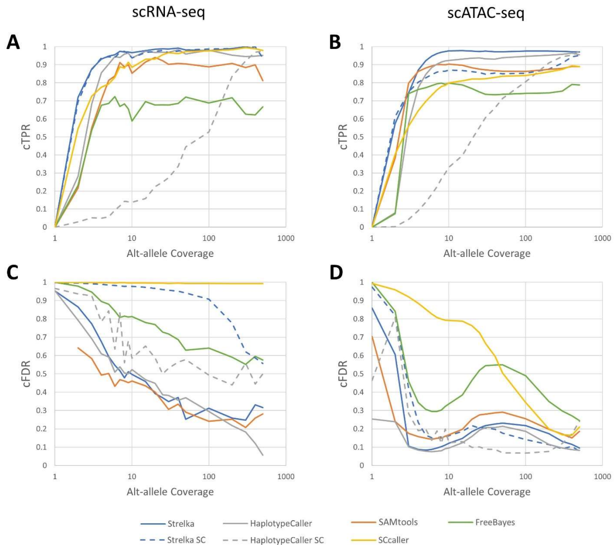
Figure 3: Average over samples of common true positive rate (cTPR) ( a, b ) and common false discovery rate (cFDR) ( c, d ) versus alternate allele coverage for variants binned by total (e.g. pooled) alt-allele coverage (e.g. the point coverage=400 would include variants from 400 to the next bin, which is 500), for each of the variant-calling approaches used, for both scRNA-seq ( a, c ) and scATAC-seq ( b, d )
