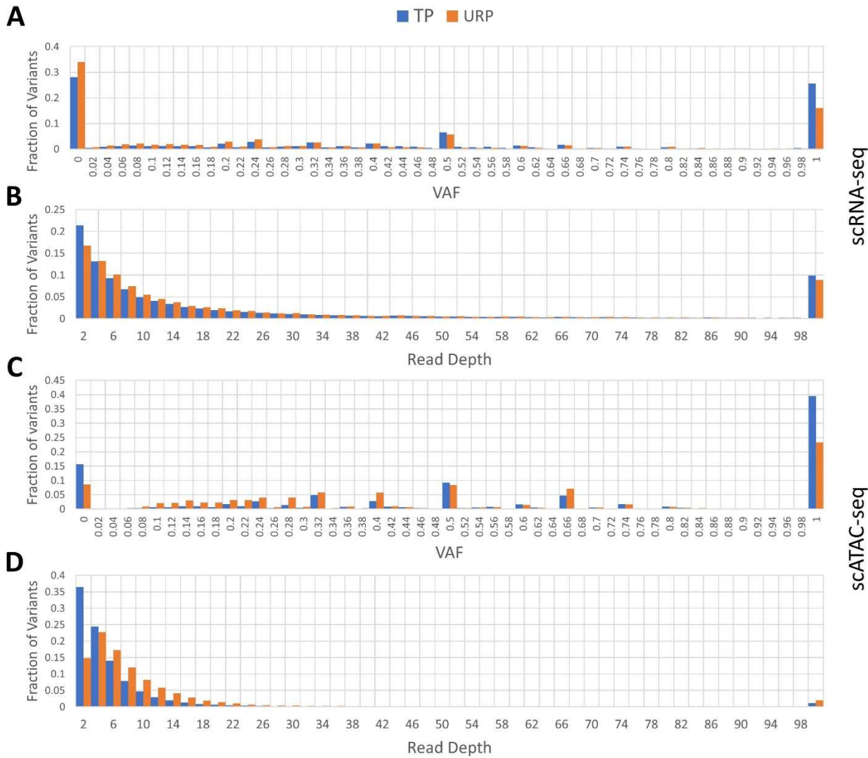
Figure 4: Comparing the composition of URP and TP variants by VAF and read depth for scRNA-seq (a, b) and scATAC-seq (c, d), number of variants with read depth over 100 are summed in the right-most bin
