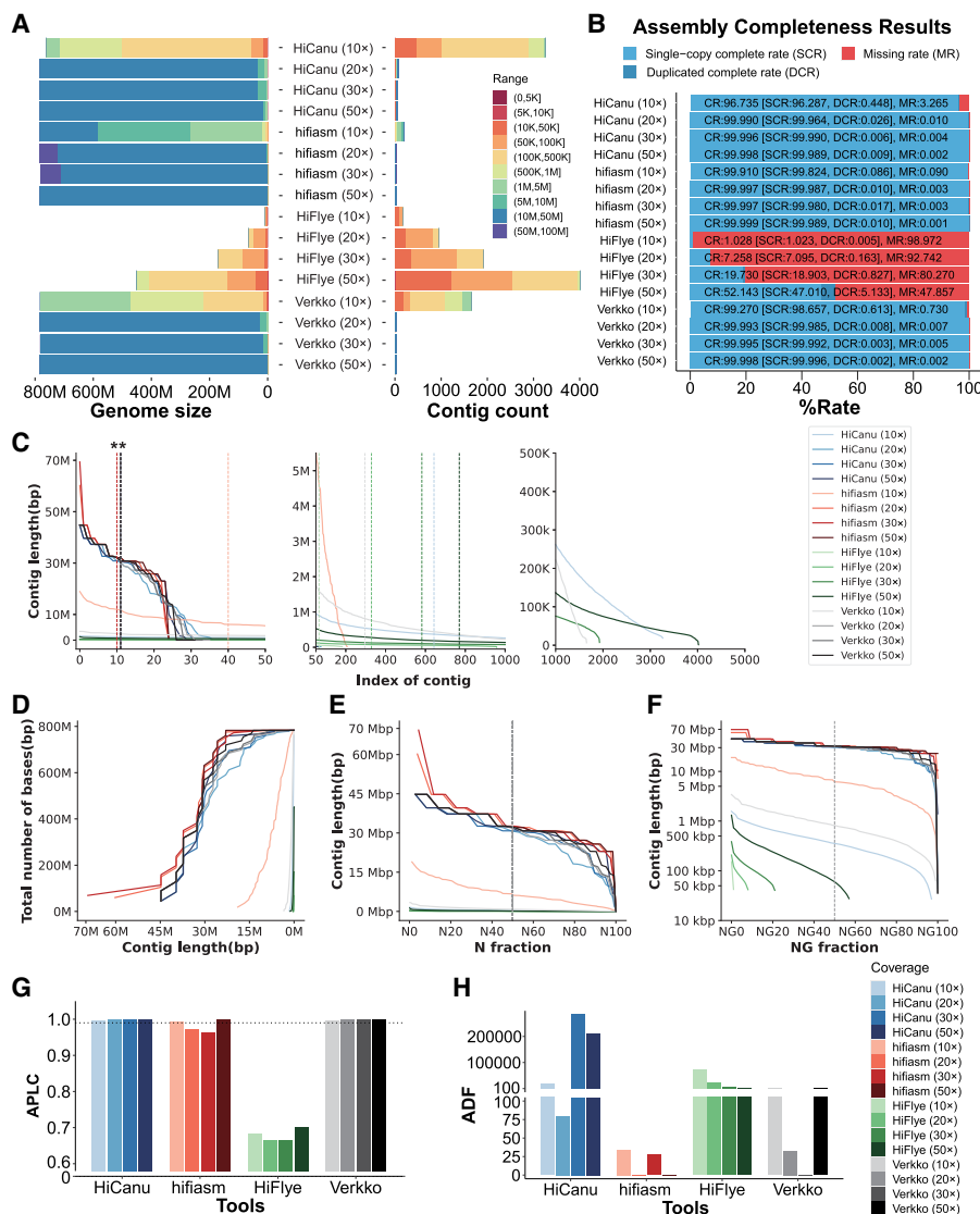
Figure 4. Summary of the performances of HiCanu, Verkko, hifiasm, and HiFlye on synthetic HiFi reads with coverage at 10x, 20x, 30x, and 50x. (A) Cumulative total size of contigs (left) and the number of contigs (right) that have a size in the range encoded by the color in the legend. (B) Single complete rate, duplicated complete rate, and missing rate. (C) Sorted contig length (left: longest 50; middle: index 50–1000; right: index 1000–5000). The horizontal lines represent the corresponding L50. (*) Overlapping data. (D) Cumulative assembly size as a function of the minimum contig length allowed in the assembly. (E) Nx length (the dashed line denotes the N50). (F) NGx length (the dashed line denotes the NG50). (G) Average proportion of largest category (APLC); the horizontal dashed line is APLC = 0.99. (H) Average distance difference (ADF).
