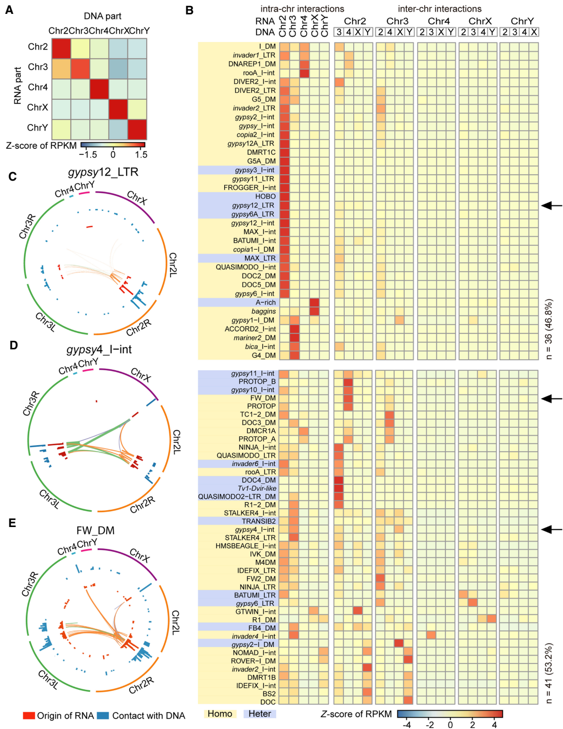
Figure 4. Cis - and trans -acting repeat-derived RNAs on chromatin. (A) Heat map of RNA–DNA interaction scores for 77 CHARRs on the same or different chromosomes. Trans -chromosome interactions are referred to as RNA interacting with DNA in chromosomes other than those from which the RNA is transcribed. (B) Assignment of each of the 77 CHARRs to either intra- or inter-chromosomal interactions in S2 cells and sorting of the data by unsupervised clustering. Top : RNA derived from different chromosomes (first row) and its DNA contacts in the same or different chromosomes (second row). The RNA–DNA interaction intensities were indicated by the z-scores according to the color key at the bottom . Arrows point to the three specific CHARRs gypsy12_LTR , gypsy4_I-int , and FW_DM , as individually illustrated in panels C–E. All CHARRs are either highlighted with yellow or blue to indicate their preferences for homotropic or heterotropic interactions, as described later. (C–E) The origins of three representative CHARRs and their DNA contacts, as shown by the Circos plots for gypsy12_LTR (C), gypsy4_I-int (D), and FW_DM (E). In each of these plots, the inner (red) track indicates the origins of individual RNAs and the outer (blue) track shows where the RNAs interact with DNA in 100-kb DNA windows. The heights of the signals correspond to reads per 100-kb window per millions. Lines specify intra- or inter-chromosomal interactions, with width suggesting the relative interaction levels in each case. The line color indicates the origin of chromatin-interacting RNAs.
