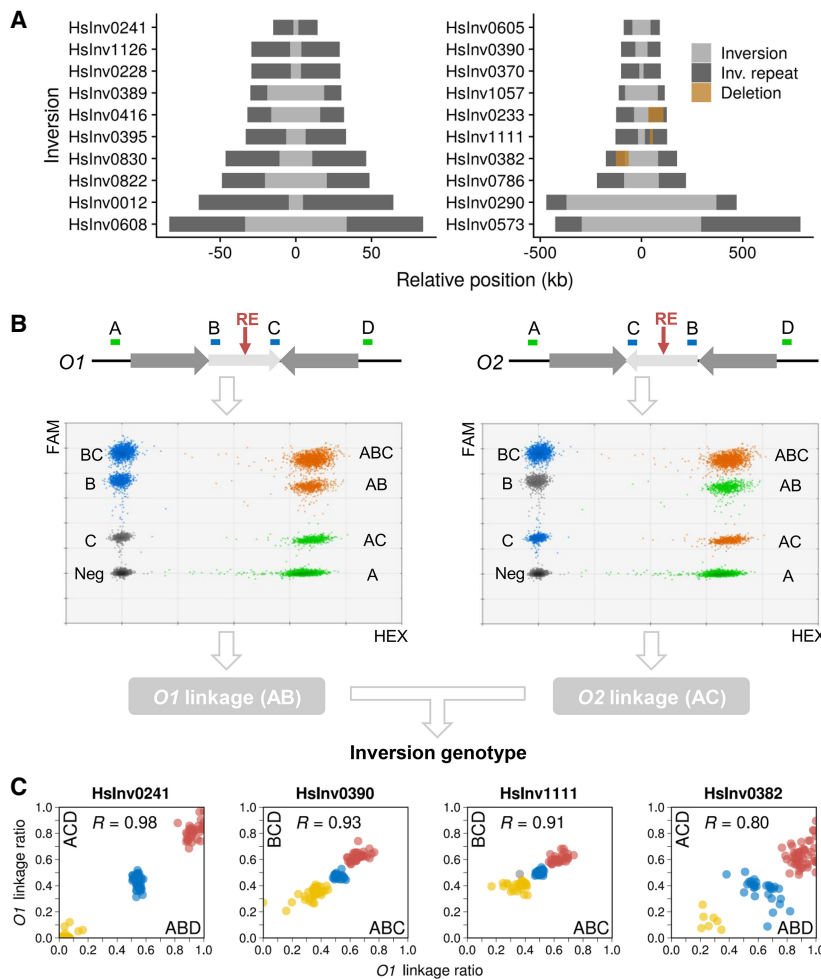
Figure 1. Inversion characterization by ddPCR genotyping. (A) Main features of the studied polymorphic inversions, with the inverted region shown in gray and the IRs as dark boxes. Brown boxes denote deletions affecting inversion breakpoints. (B) Strategy for ddPCR genotyping of an inversion (light gray arrow) mediated by IRs at inversion breakpoints (dark gray arrows) using as an example the simultaneous triplex amplification of amplicons A, B, and C (shown on top), although the same procedure was used for other amplicon combinations (BCD, ABD, or ACD). O1 linkage (AB, left) and O2 linkage (AC, right) were calculated separately from the triplex ddPCR results, ignoring, respectively, amplicons C (left graph) or B (right graph). Colors of droplet clusters indicate if they are used to estimate the molecules containing only amplicon A (green), only the B or C internal amplicon (blue), two amplicons at the same time, either A and B or A and C (orange), or if they are considered as negative (gray). (C) Plots of O1 linkage ratios obtained from two different triplex ddPCR reactions (indicated in each axis) interrogating both breakpoints of four inversions in 95 analyzed individuals and the correlation between them ( R ), which show clearly differentiated genotype groups ( O1/O1 , red; O1/O2 , blue; O2/O2 , yellow). HsInv0241, where DNA was digested to separate both breakpoints with a restriction enzyme (RE, red arrow in B), shows the expected linkage ratios, but homozygote and heterozygote clusters are closer in HsInv0390, HsInv1111, and HsInv0382 analyzed using undigested DNA. The effect of a large deletion within breakpoint AB in HsInv0382 can be seen as higher O1 linkage ratio values in the horizontal axis. The gray dot is a sample with altered amplicon ratios in HsInv1111 ABC breakpoint.
