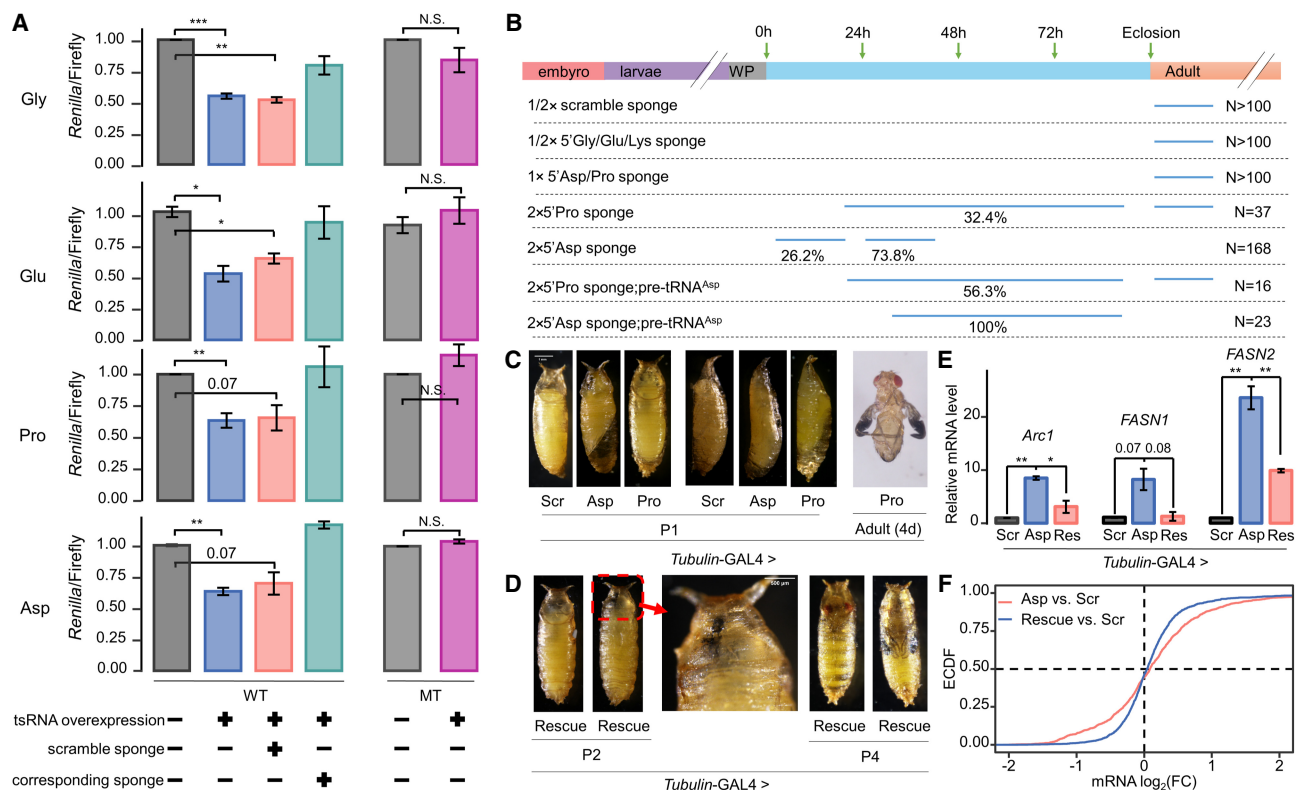
Figure 5. Evaluation of regulatory activities of 5'-tsRNAs in vitro and during development. (A) Normalized Renilla/Firefly reporter activities to assay target site-dependent regulation by 5'-tsRNAs. WT: Renilla reporter gene carrying three target sites of each tsRNA. The sequences were cloned from native genes carrying predicted target sites (Supplemental Fig. S9B). MT: Renilla reporter gene carrying three sites with scrambled sequences in the seed match. For 5'-tsRNA GlyGCC , 5'-tsRNA GluCUC , and 5'-tsRNA ProUGG , the sites were placed in 3' UTR; for 5'-tsRNA AspGUC , the sites were placed in CDS with the consideration of their higher inhibitory effects (Supplemental Fig. S7C). tsRNA overexpression: synthetic tsRNA mimic and the pAWH vector to express the corresponding pre-tRNA. tsRNA sponge: synthetic RNA sequence that is reversely complementary to the tsRNA. Scramble sponge: synthetic RNA sequence that is randomly scrambled from the sponge. See Supplemental Tables S2–S5 for the sequences. (B) Summary of the estimated lethality time based on the stage at which pupae stopped developing. For 5'-tsRNA GlyGCC , 5'-tsRNA GluCUC , 5'-tsRNA LysUUU , and the scramble 5'-tsRNA AspGUC , Tubulin-GAL4 -driven one or two copies of sponge elements did not show any observable phenotypes (N>100). For Tubulin-GAL4 -driven one copy of sponge element against 5'-tsRNA AspGUC and 5'-tsRNA ProUGG , some mild traits were observed but all pupae emerged (N>100). (C) The pupal lethality phenotype of Tubulin-GAL4 -driven two copies of sponge elements against 5'-tsRNA AspGUC and 5'-tsRNA ProUGG . All 5'-tsRNA AspGUC -sponge pupae ("Asp"; N = 168) did not survive beyond P2. 26.2% of them had an abnormal body curvature and died during P1. 73.8% showed a failure in head inversion and an improper air bubble location during P2. The 5'-tsRNA ProUGG -sponge pupae ("Pro"; N = 37) showed high phenotypic heterogeneity. 32.4% of them proceeded through P1 but failed to eclose. 67.6% emerged with various defects such as un-spread wings 4 d after emergence. The Tubulin-GAL4 -driven two copies of scramble sponge ("Scr") was used as control, and all tested pupae (N>100) emerged without observable defects. (D) Phenotypic rescue with pre-tRNA AspGUC . All rescued pupae ("Rescue"; N = 23) proceeded through P1 with finished head evert process and correct air bubble location. 43.5% of them lived to P4 as late pharate adults, but had leg malformation and did not eclose. (E) qRT-PCR confirming that the mRNA levels of three selected 5'-tsRNA AspGUC target genes were restored by pre-tRNA AspGUC . All samples were collected from P1 pupae. Arc1 , FASN1 , and FASN2 were selected because of their known expression and function during the larva-to-pupa transition. rp49 was used as internal control. Each experiment had two independent replicates. Error bars represent SEM, and Student's t -tests were used. (F) mRNA-seq confirming that the mRNA levels of 5'-tsRNA AspGUC target genes (N = 1411) were restored by pre-tRNA AspGUC . Kolmogorov–Smirnov test P -value = 10^{-11} .
