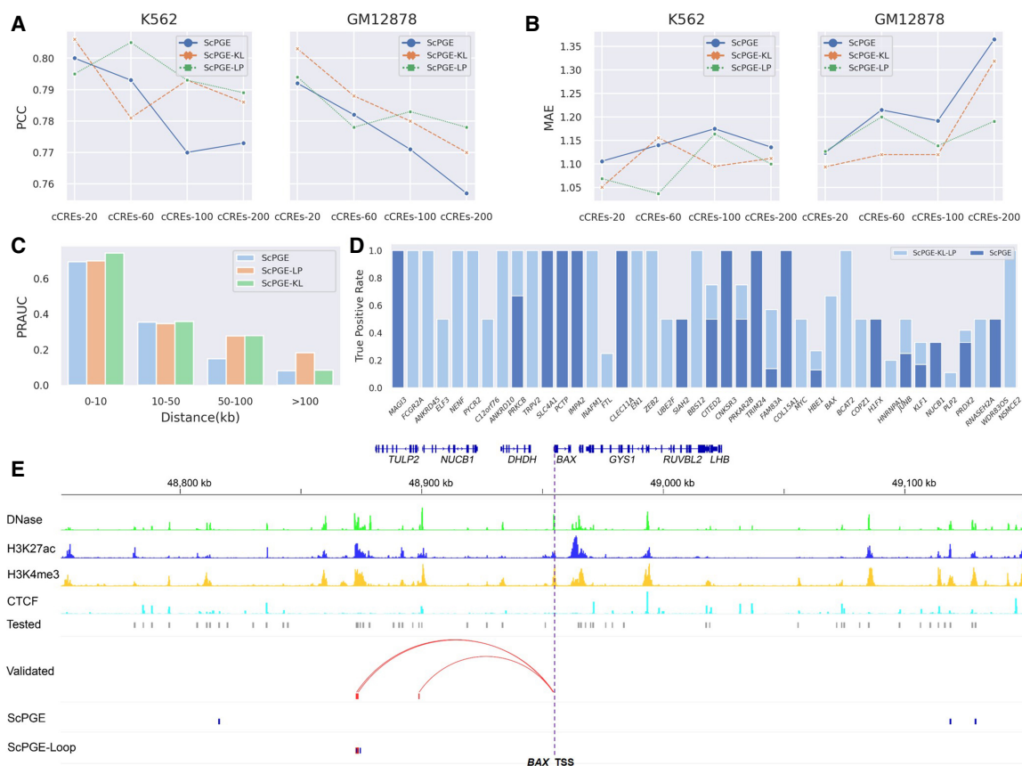
Figure 5. Chromatin loops facilitate ScPGE to capture cCRE-gene interactions. (A,B) Comparison of the performance of ScPGE, ScPGE-KL, and ScPGE-LP as the number of cCREs increases. (C) The performance (PRAUC) of ScPGE, ScPGE-KL, and ScPGE-LP in classifying cCRE-gene pairs at different distance groups. (D) The true positive rates of ScPGE and ScPGE-Loop on validated cCREs. (E) Visualization of active cCREs of the BAX gene missed by ScPGE but identified by ScPGE-Loop, where validated cCREs are represented by red rectangles and correctly identified cCREs are represented by blue rectangles with red outlines.
