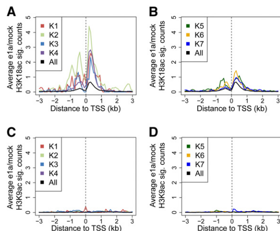
Figure 4. Relationship of the RB-binding clusters to histone acetylation change. (A,B) Average significant (sig.) counts of change in H3K18ac levels in d /1500- versus mock-infected cells are shown for the seven RB-clusters (see Fig. 3C). (C,D) Average significant (sig.) counts of change in H3K9ac levels in d /1500- versus mock-infected cells are shown for the seven RB-clusters (see Fig. 3C).
